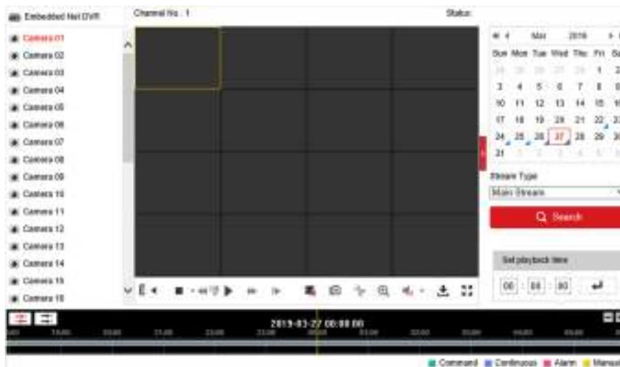
Figure 9-3 Playback
