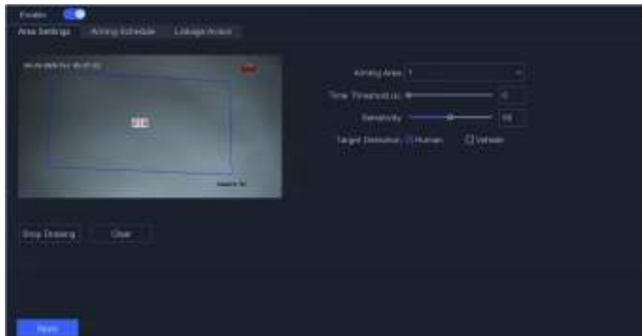
Figure 5-12 Intrusion Detection
