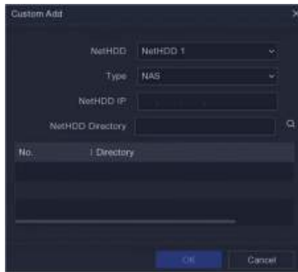
Figure 5-16 Add NetHDD
