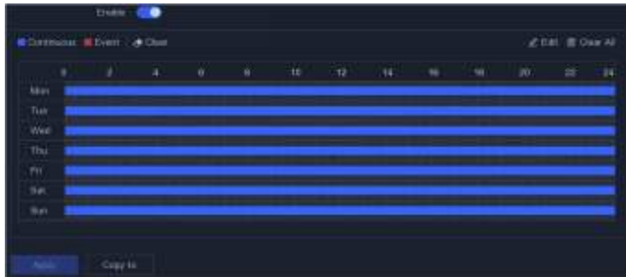
Figure 5-17 Recording Schedule
