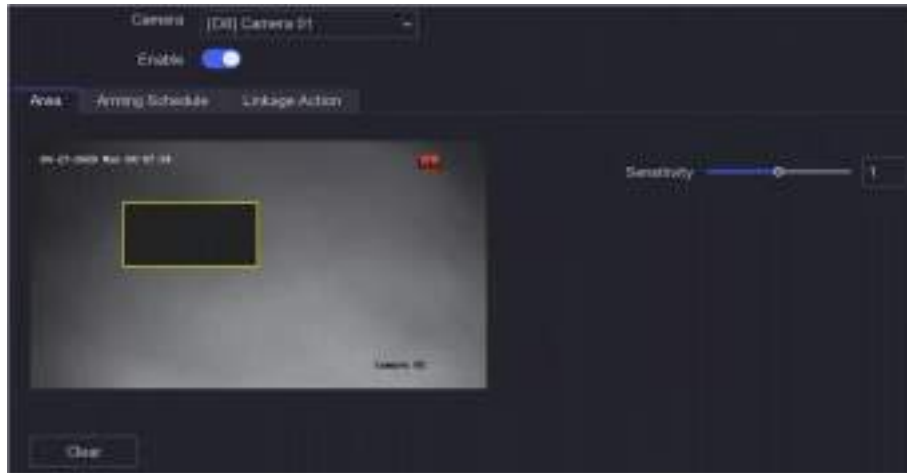
Figure 6-15 Video Tampering
